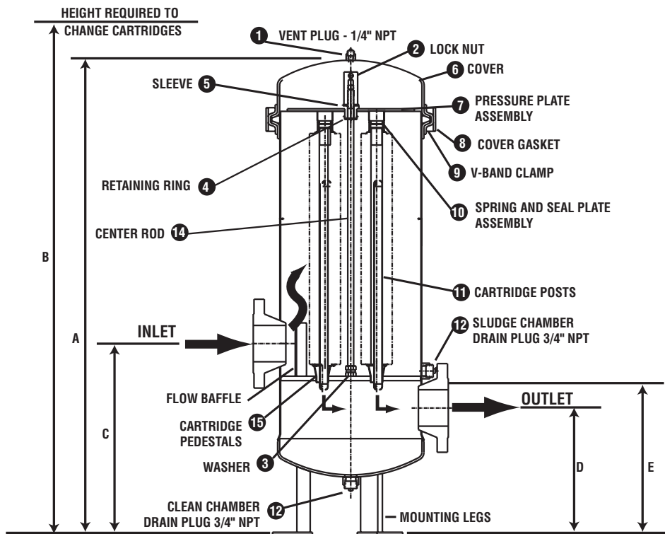
Elevation View
