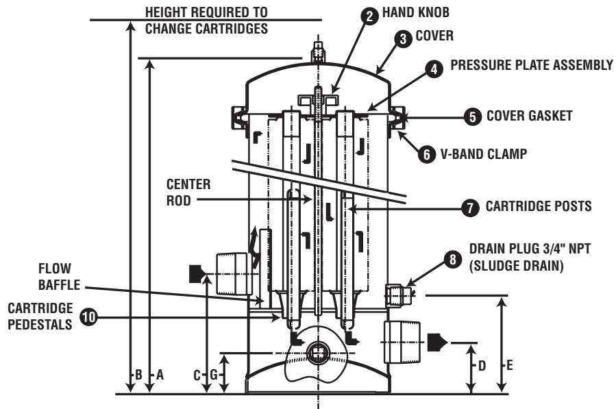
Elevation View
