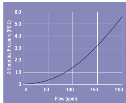
Graph 1: Flow vs. Differential Pressure
