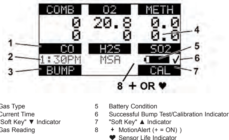
Figure 2-2. Monochrome Display
