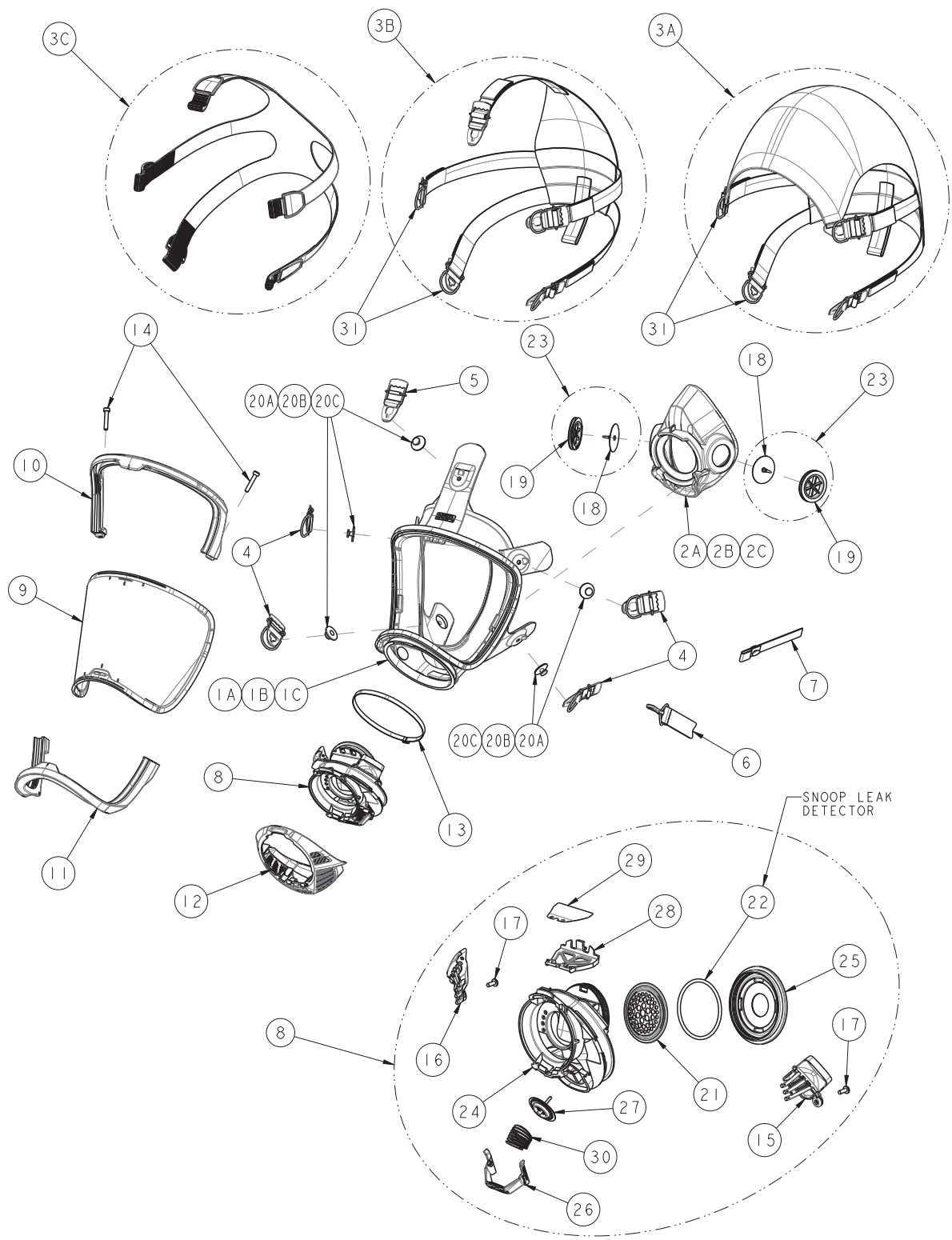
Fig. 10 Exploded View
