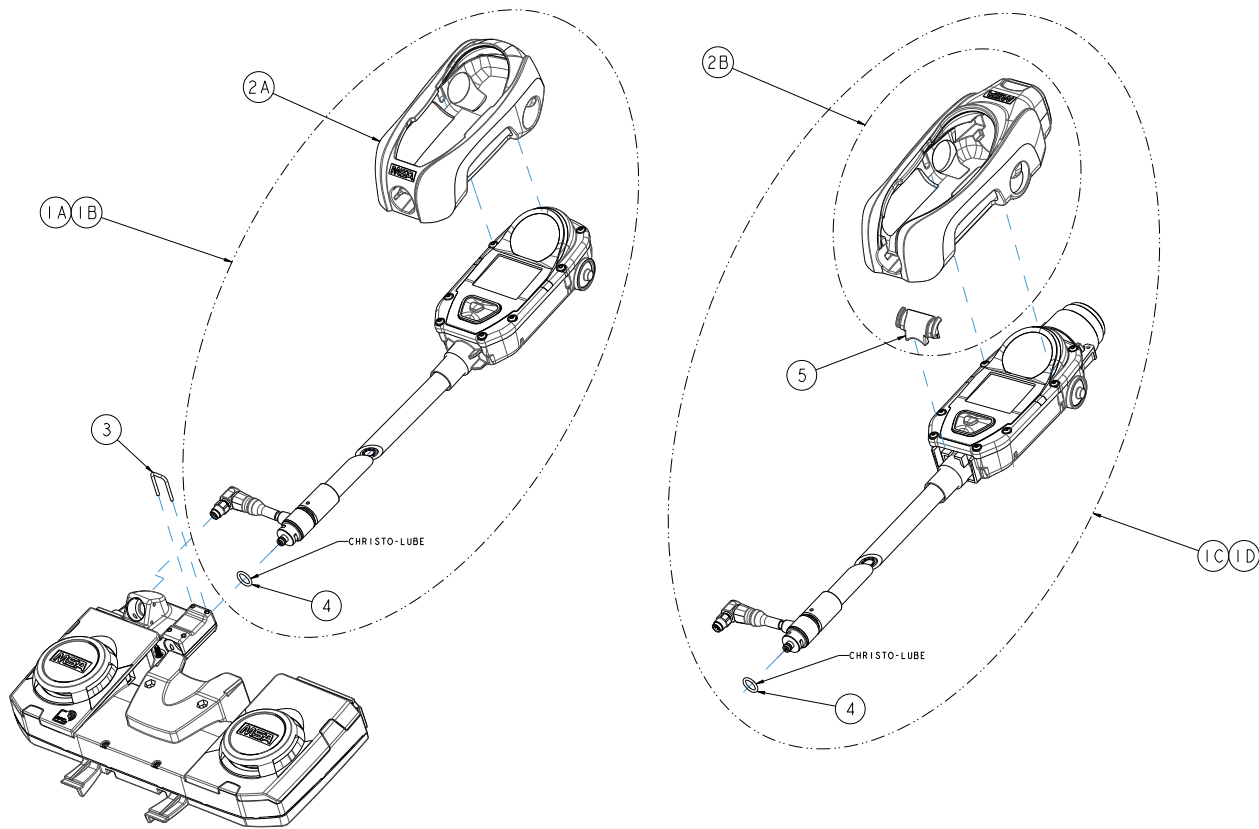
Fig. 2 Exploded View
