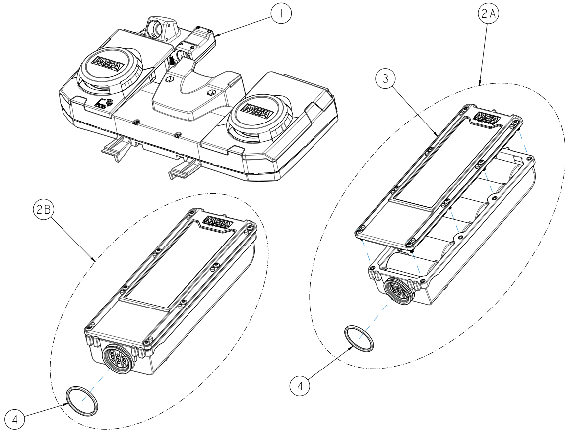
Fig. 3 Exploded View
