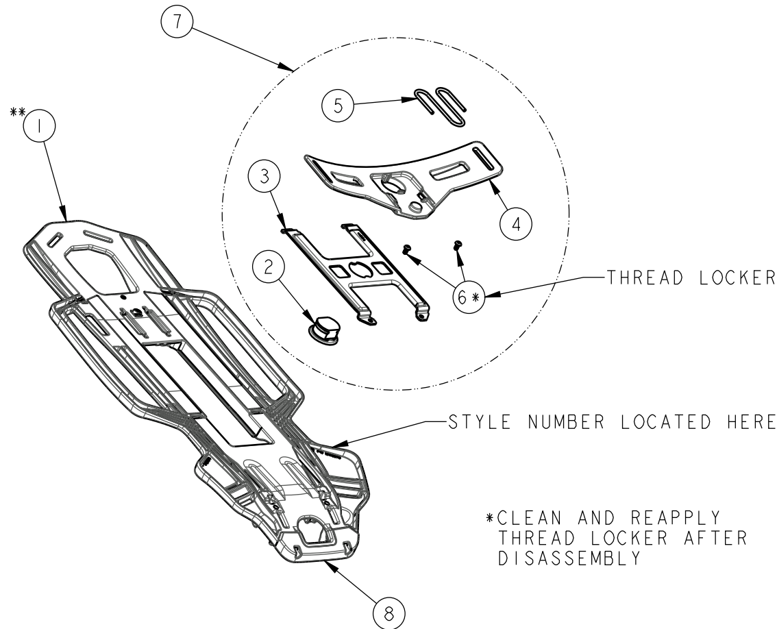
Fig. 5 Exploded View - FIXED SWIVEL LUMBAR
