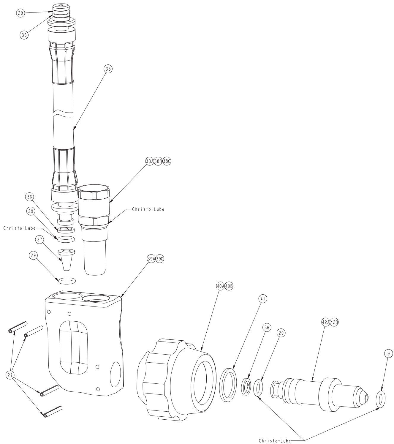
Fig. 13 G1 Remote Threaded Connect Handwheel
