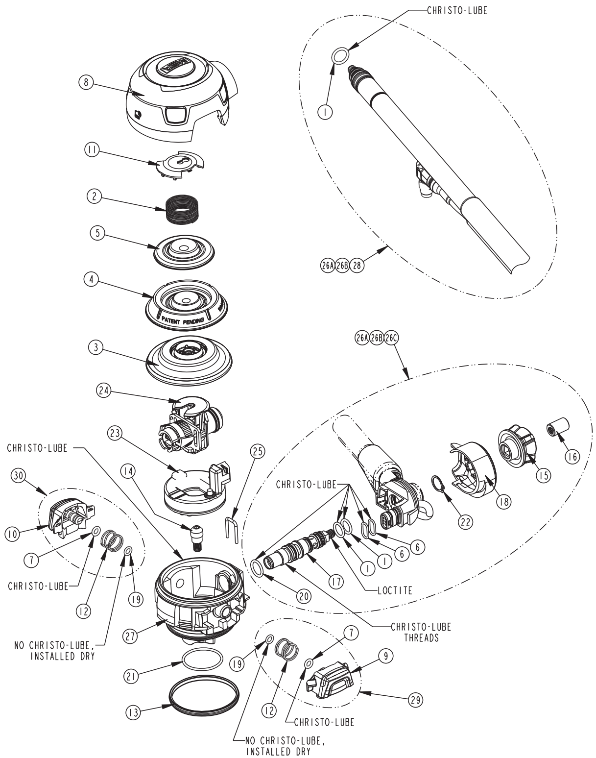
Fig. 11 Exploded View
