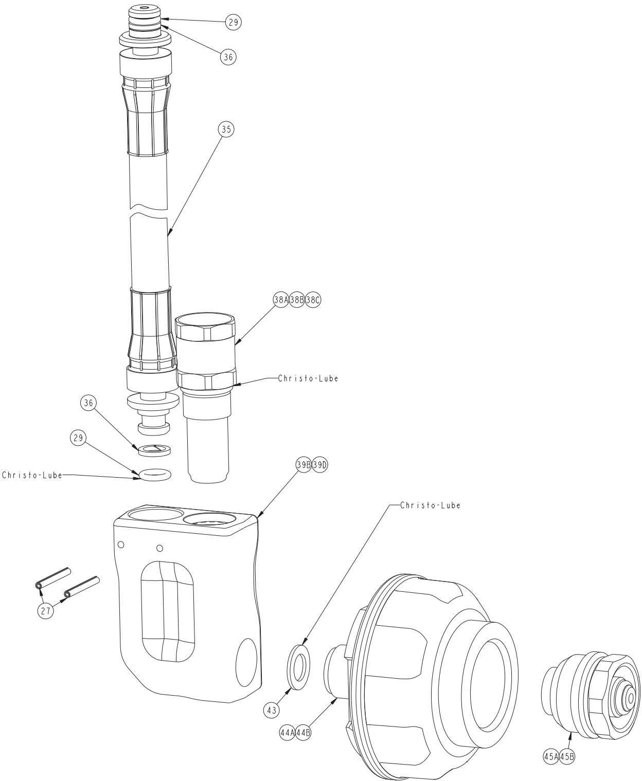
Fig. 14 G1 Remote Quick Connect Handwheel
