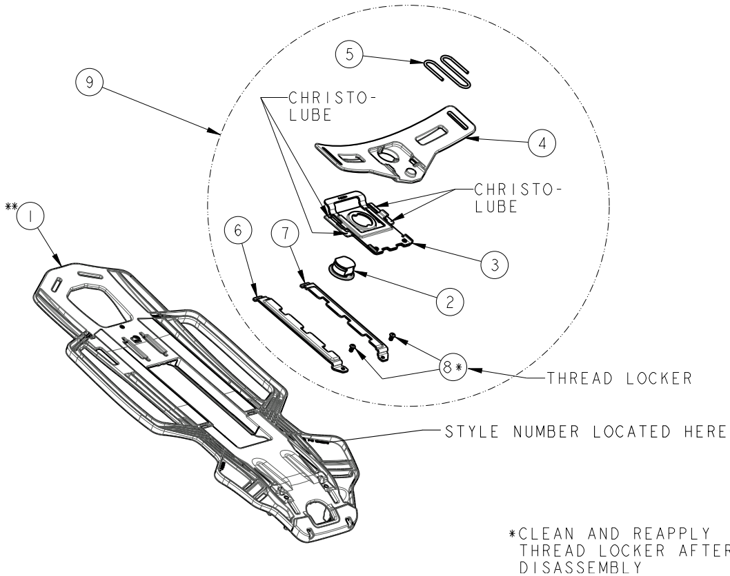
Fig. 6 Exploded View - ADJUSTABLE SWIVEL LUMBAR
