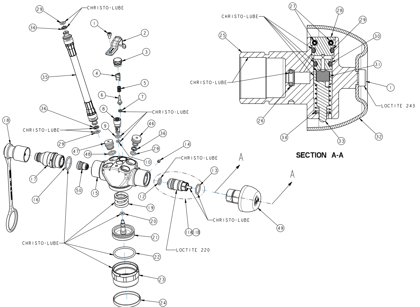
Fig. 12 Exploded View - Pressure reducer
