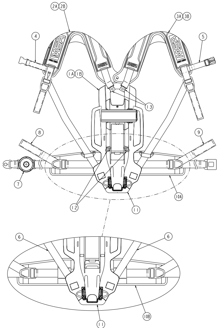
Fig. 4 Exploded View - Harness and Backplate
