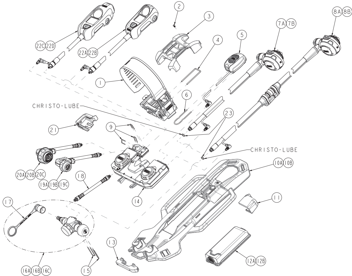
Fig. 1 Exploded View - Primary Subsystem Connections
