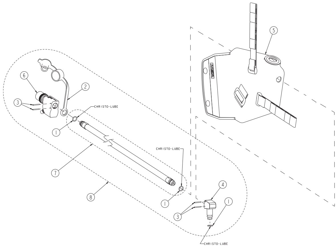
Fig. 15 Exploded View
