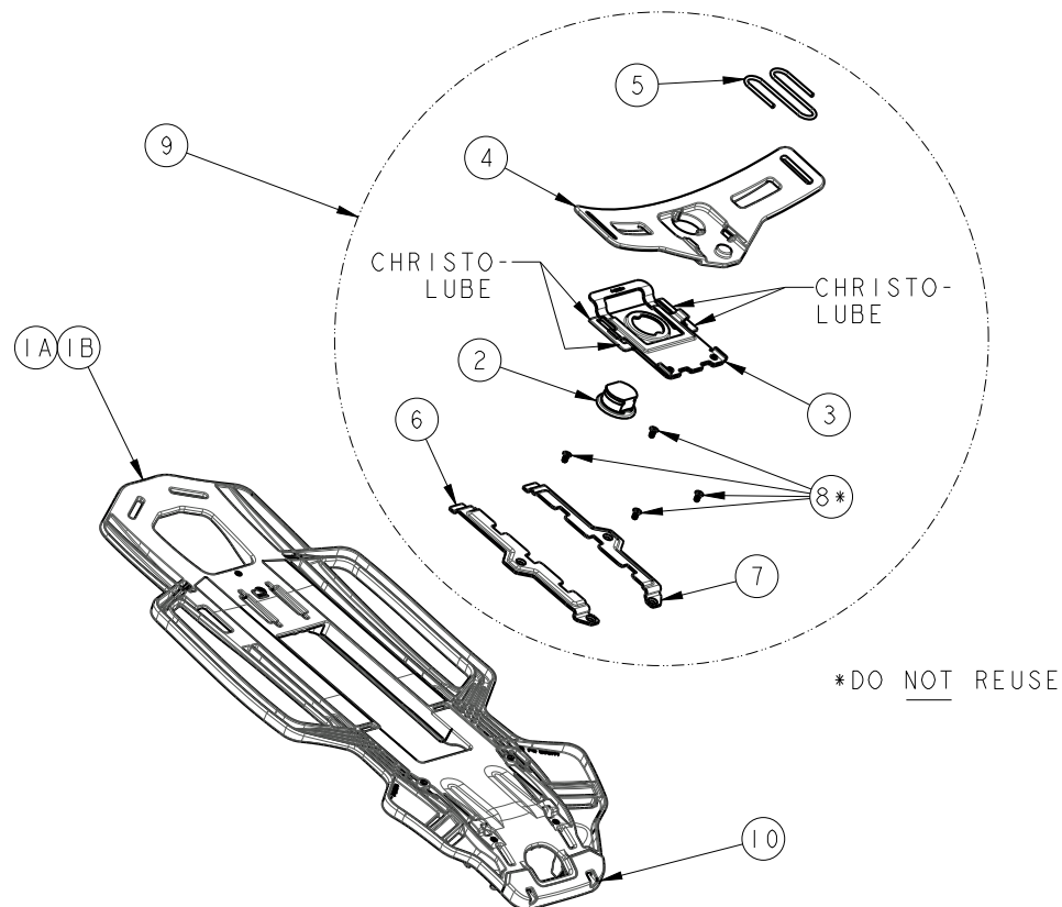
Fig. 7 Exploded View - ADJUSTABLE SWIVEL LUMBAR
