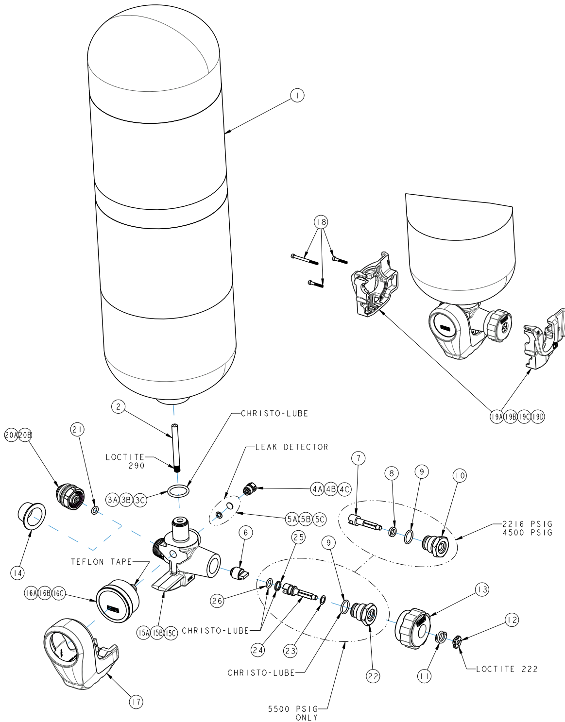
Fig. 9 Exploded View
