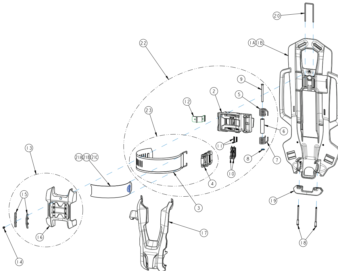
Fig. 8 Exploded View - METAL BAND
