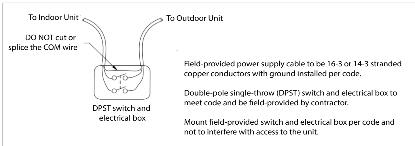
Figure 1. Disconnect Installation
