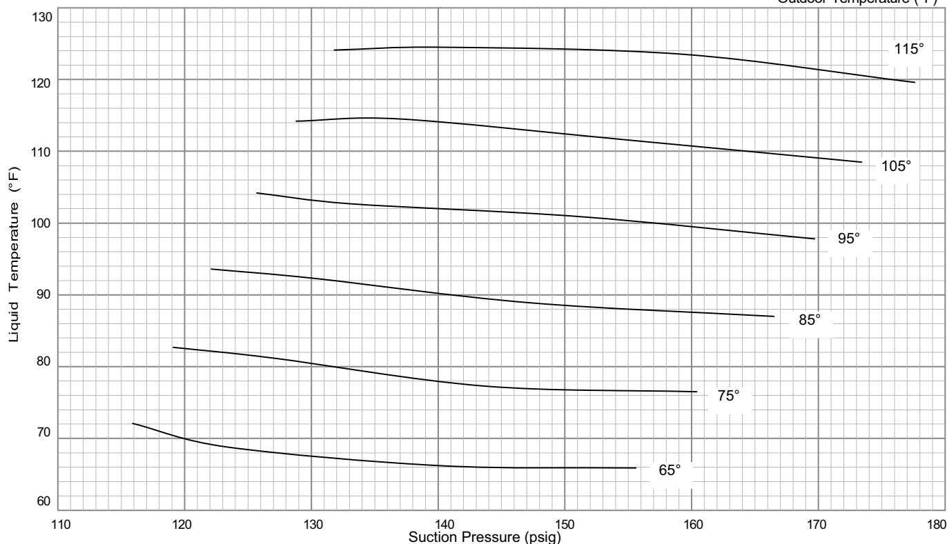
ZGB/ZCB036 CHARGING CURVE - ALL-ALUMINUM COIL
