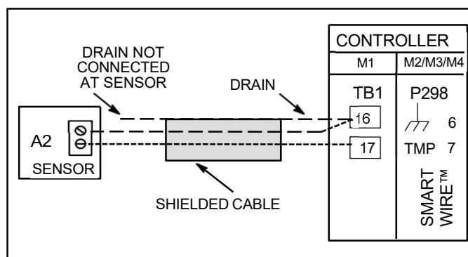
Figure 1. Sensor Wiring
