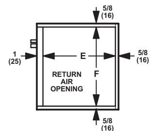
END VIEW
