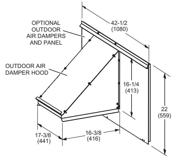
END VIEW
