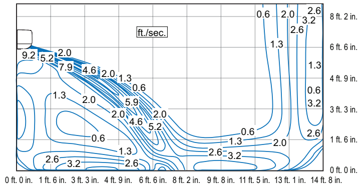
MWCB012S4 - COOLING
