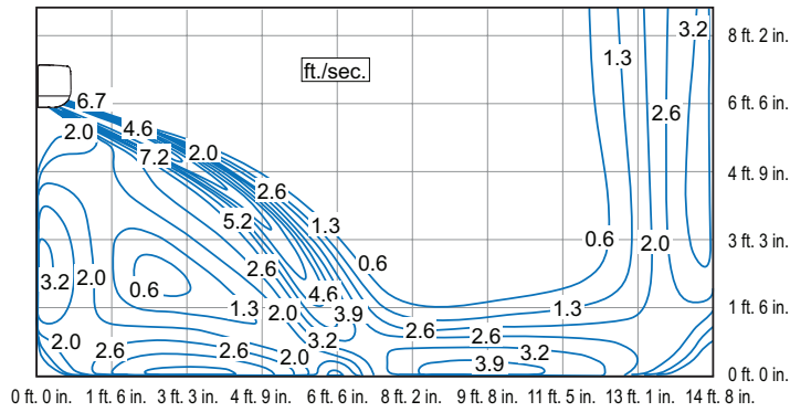
MWCB009S4 - COOLING
