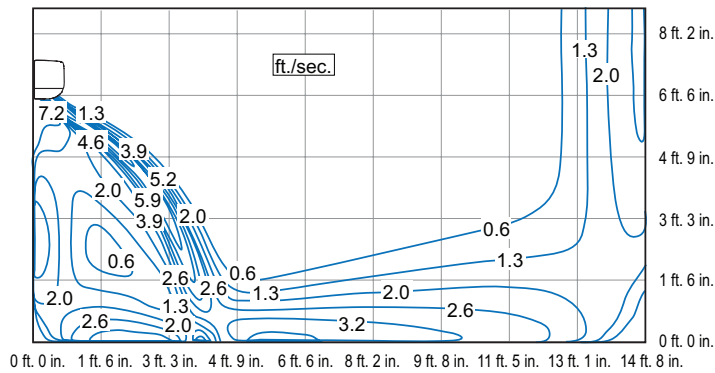
MWCB018S4 - COOLING
