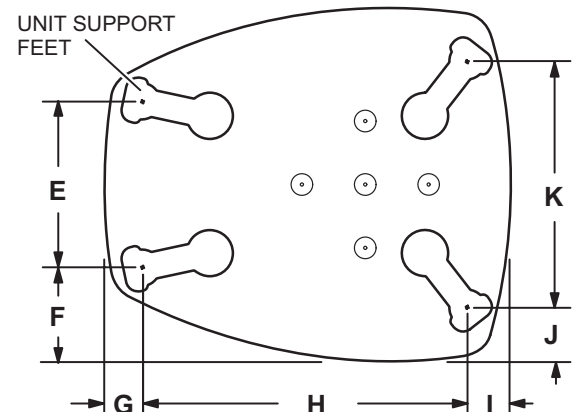
048 AND 060 BASE SECTION (Medium and Large Base)
