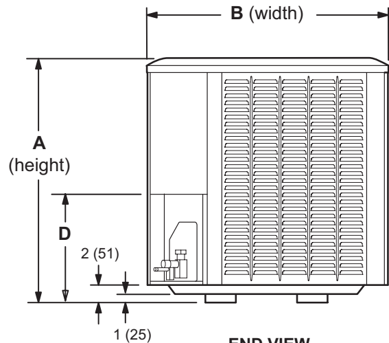
END VIEW
