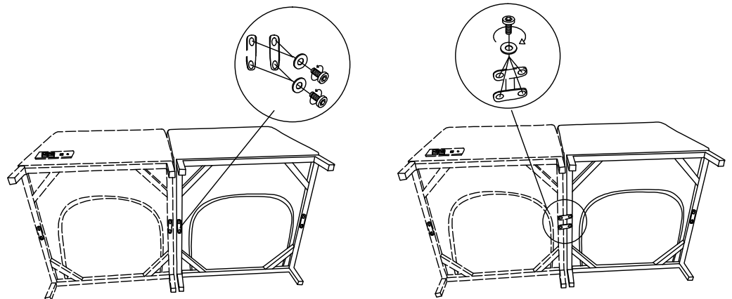
1/4"×2" SCREW – QTY: 4
