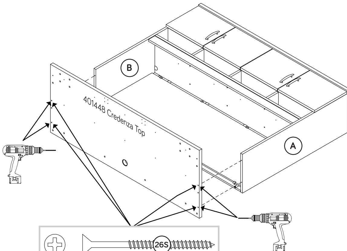
BLACK 2-1/4" FLAT HEAD SCREW (4 used in this step)
