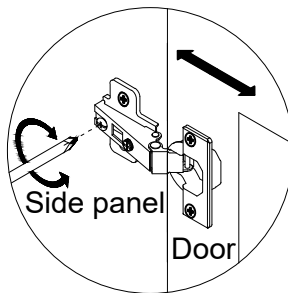
ADJUSTMENT DEPTH
