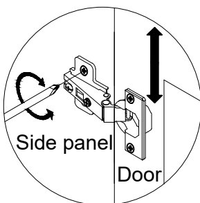
ADJUSTMENT HEIGHT
