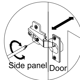
ADJUSTMENT GAP
