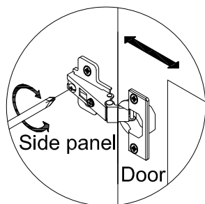
ADJUSTMENT DEPTH
