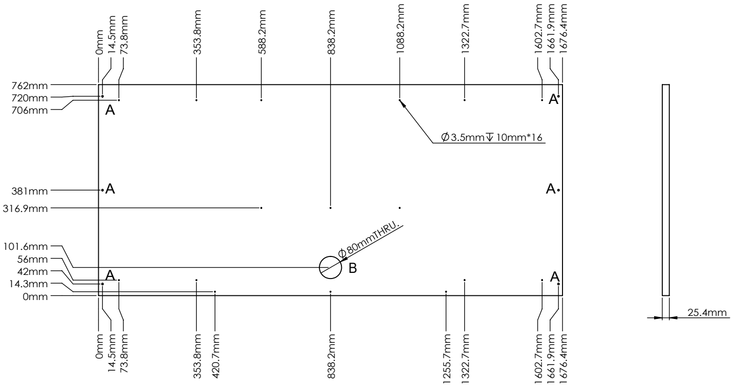
Bottom View
