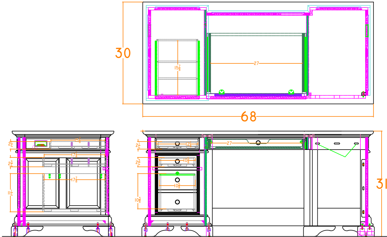
I224-307 Computer Desk 68"W x 30"D x 31"H
