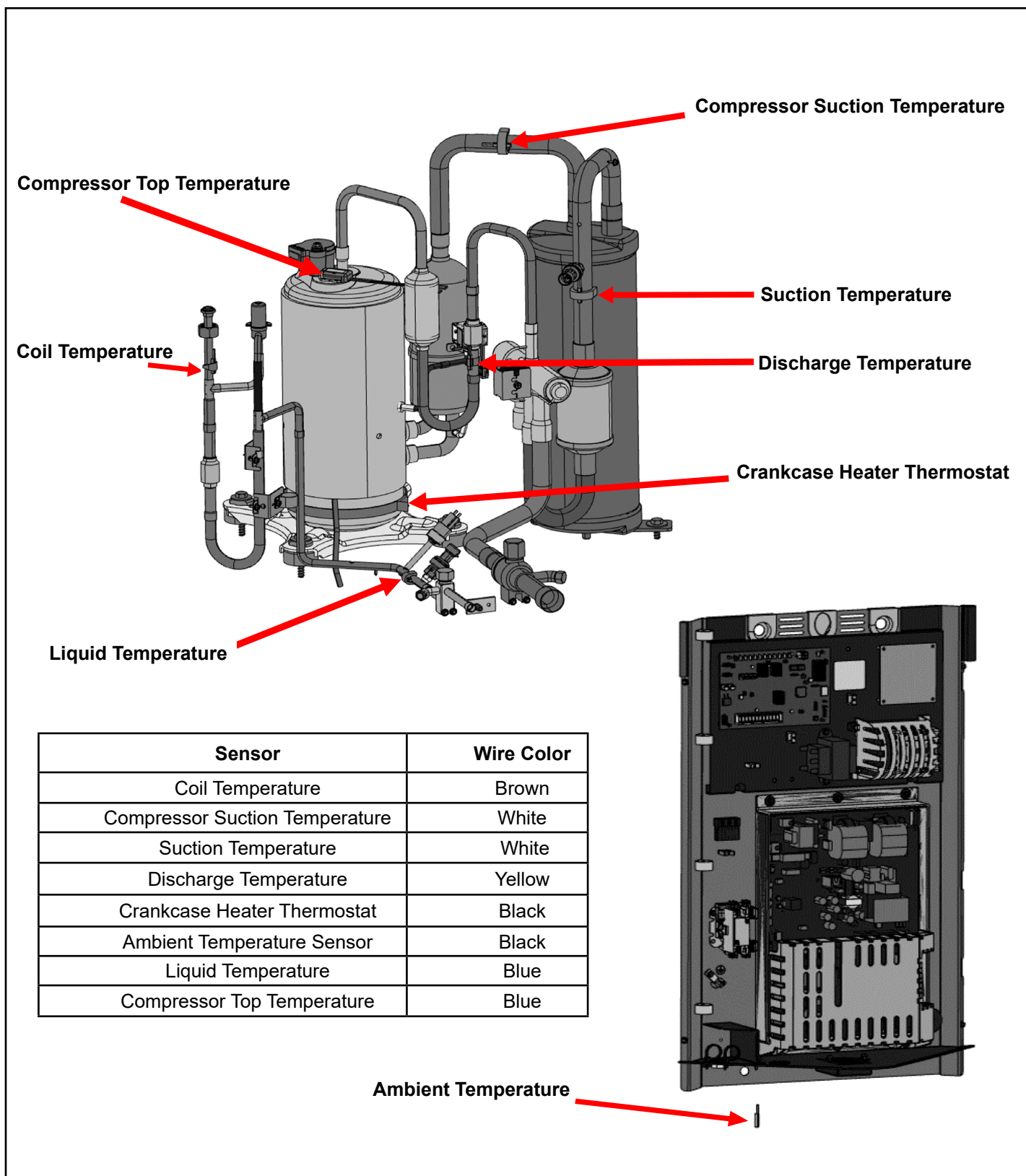
FIGURE 12. Temperature Sensor Locations
