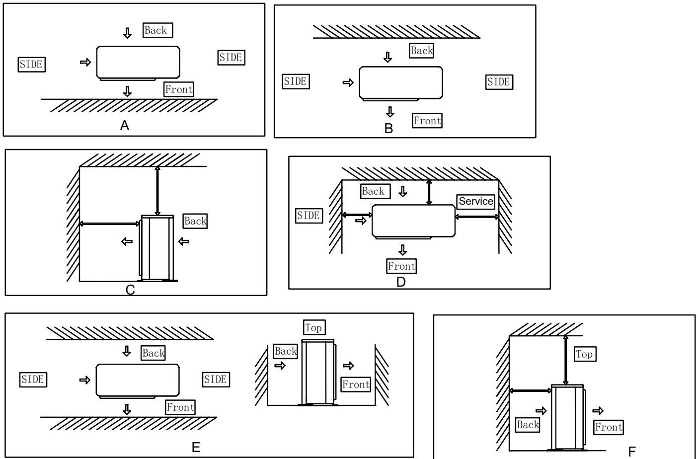
Figure 1. Single-Unit Clearance Configurations
