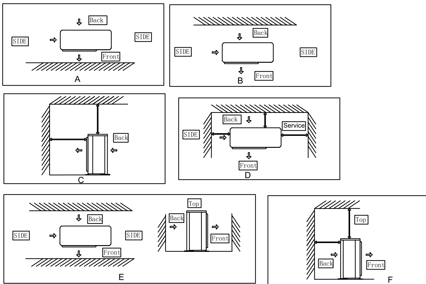
Figure 1. Single-Unit Clearance Configurations
