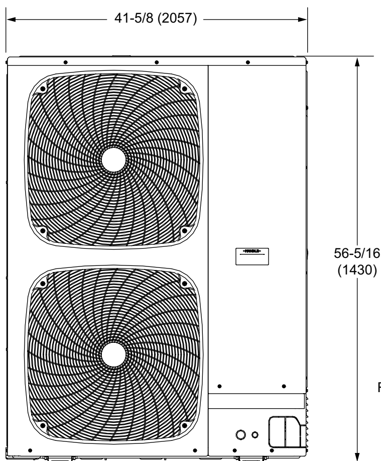
FRONT VIEW
