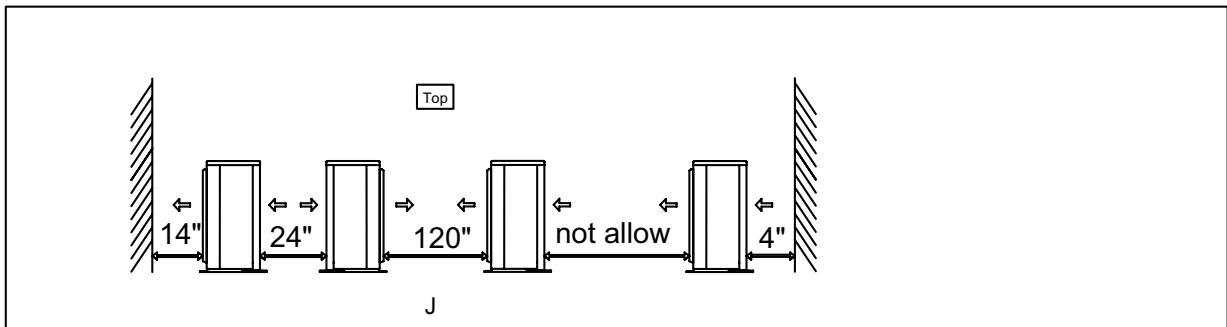
Figure 2. Multiple-Unit Clearance Configurations
