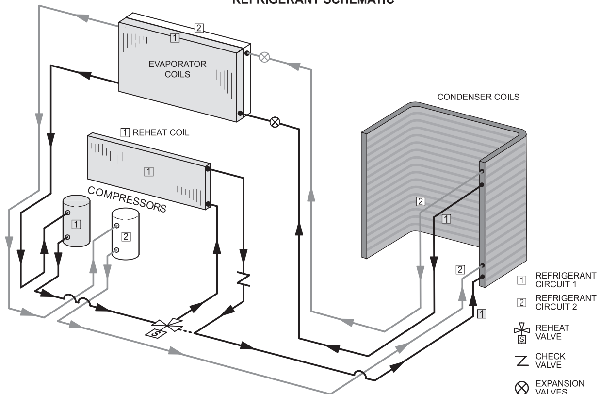
REFRIGERANT SCHEMATIC
