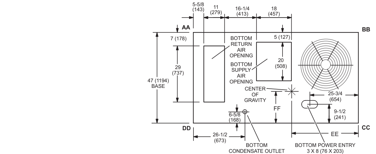
TOP VIEW (Base)
