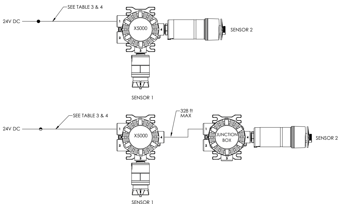
Fig. 29 Two Sensors
