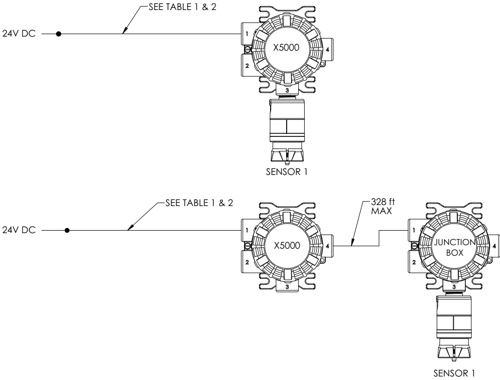
Fig. 28 Single Sensor
