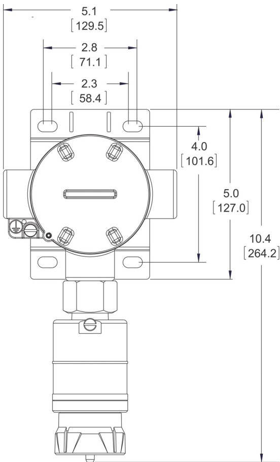
Fig. 55 M25 JB5000 Dimensions with Digital Sensor
