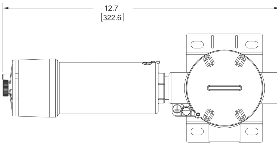
Fig. 57 JB5000 Dimensions with XIR PLUS
