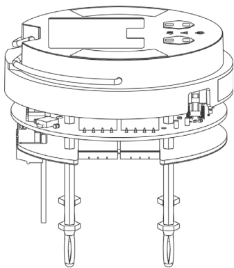
Fig. 37 Relay Board Stack
