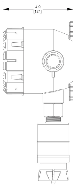
Fig. 52 Deep Lid Depth with M25 Adapter
