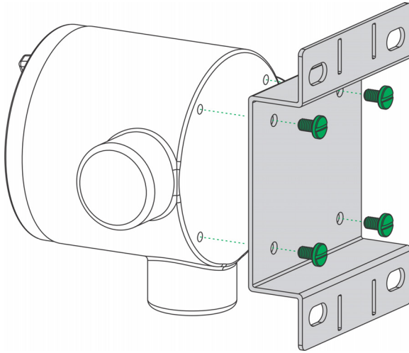
Fig. 17 JB5000 bracket attachment
