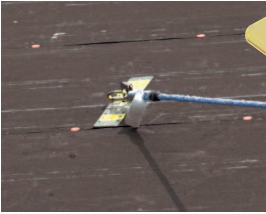
Reusable Roof Anchor installed off roof peak
