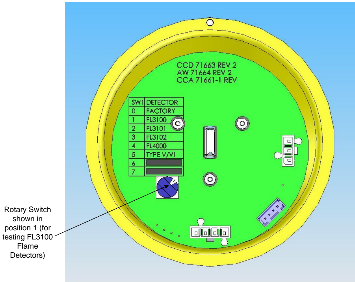
Figure 5: Location of Functional Board under Lamp Assembly
