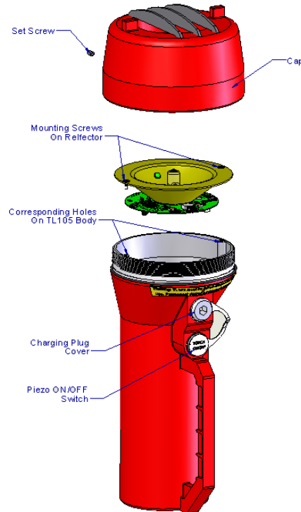
Figure 4: Reflector Mounting in Body
