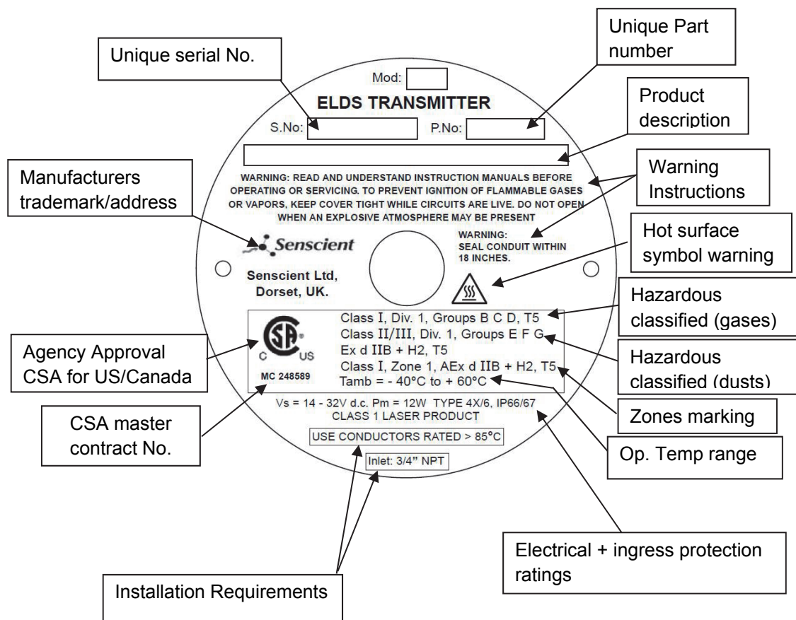
Label for Tx Unit (Receiver is Similar) Note
