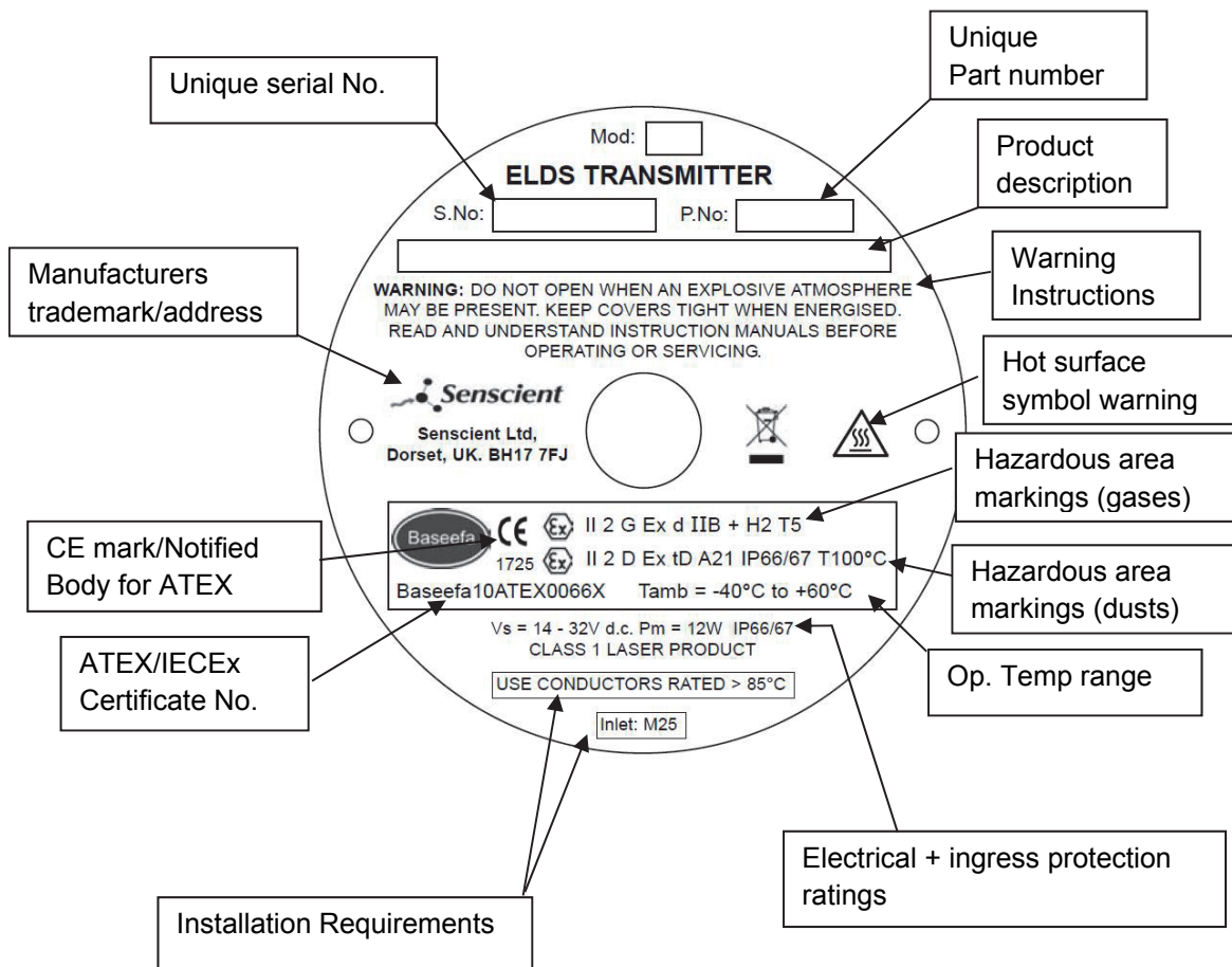
ATEX Certification Label for Tx Unit (Receiver is Similar)
