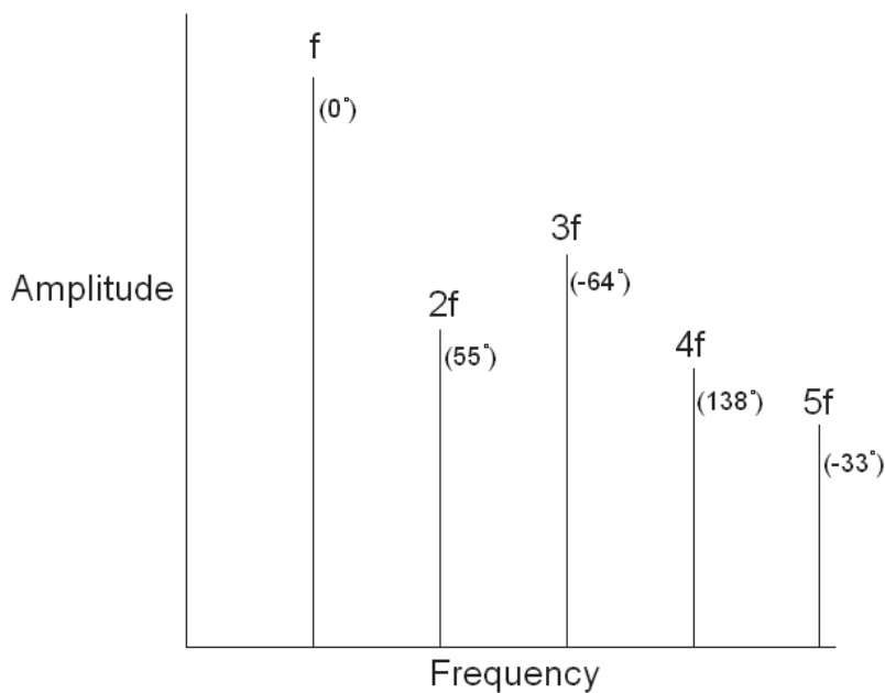
Harmonic Fingerprint for a H 2 S Line at 1589.97nm
