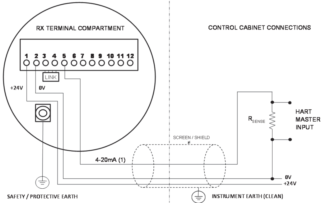
RX WIRING DIAGRAM: HART 4-20 (1) SOURCE
