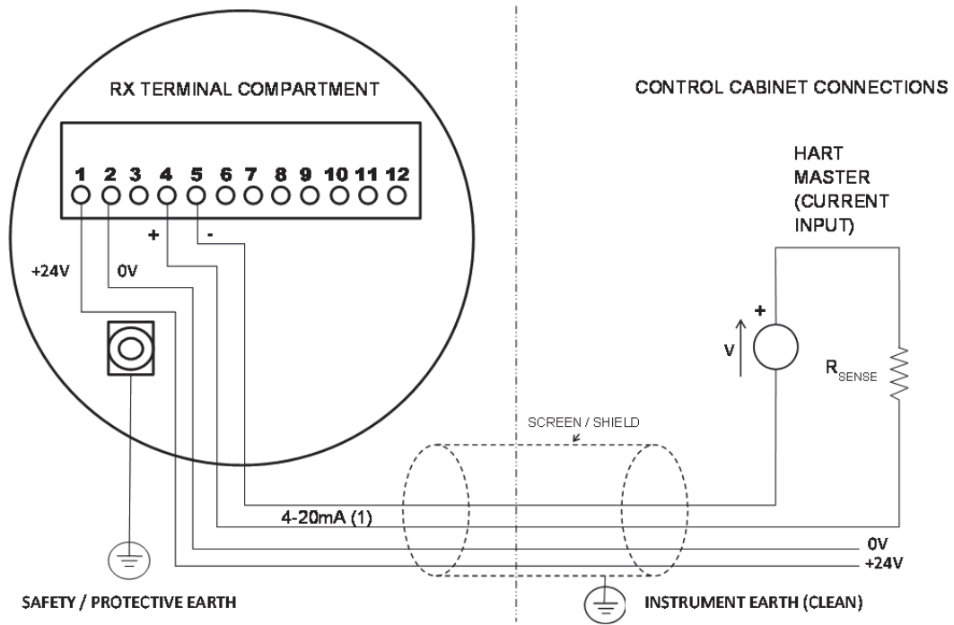
RX WIRING DIAGRAM: HART 4-20 (1) ISOLATED
