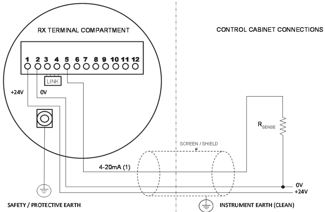
Wiring Diagram for ELDS 1000 Receiver with Current Sink @ 4-20 (1)
