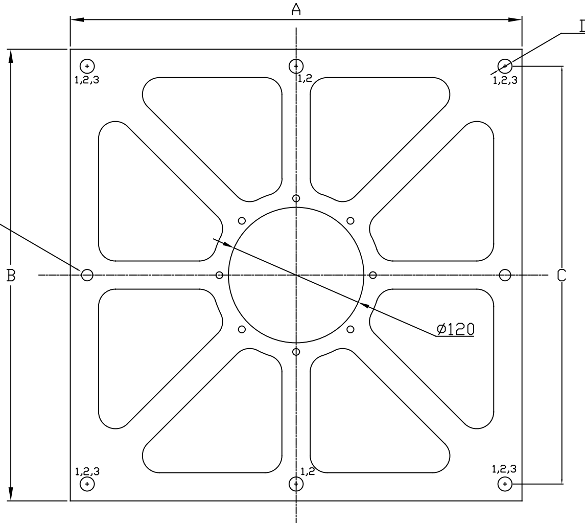
Image shows High Temperature Mounting Plate (400x400)
