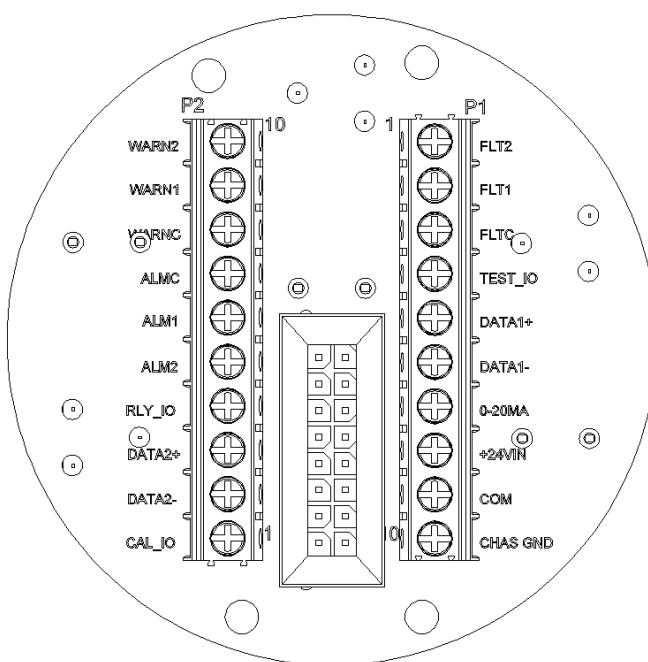
Figure 20: Terminal Connections 7
