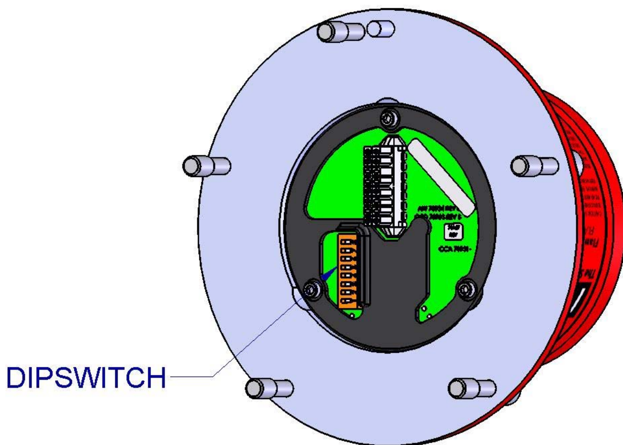
Figure 23: Dipswitch Location
