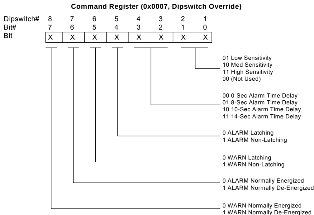
Figure 24: Command Register
