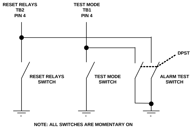
Figure 22: Wiring Diagram – Reset Relays, Test Mode, & Alarm Test
