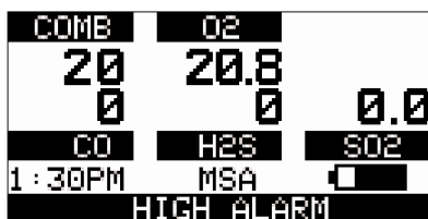
Figure 2-6. Alarm Conditions (High Alarm shown)
