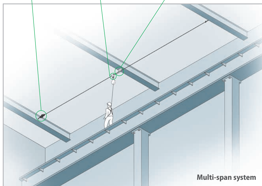
Typical uses of overhead systems illustrated: rail car loading bay (top) and internal factory access (below).
