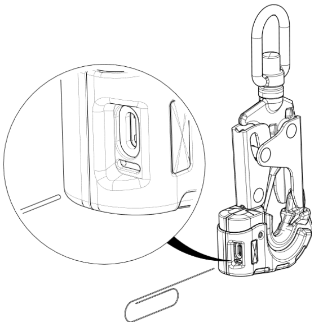
Figure 4 Reset io1
