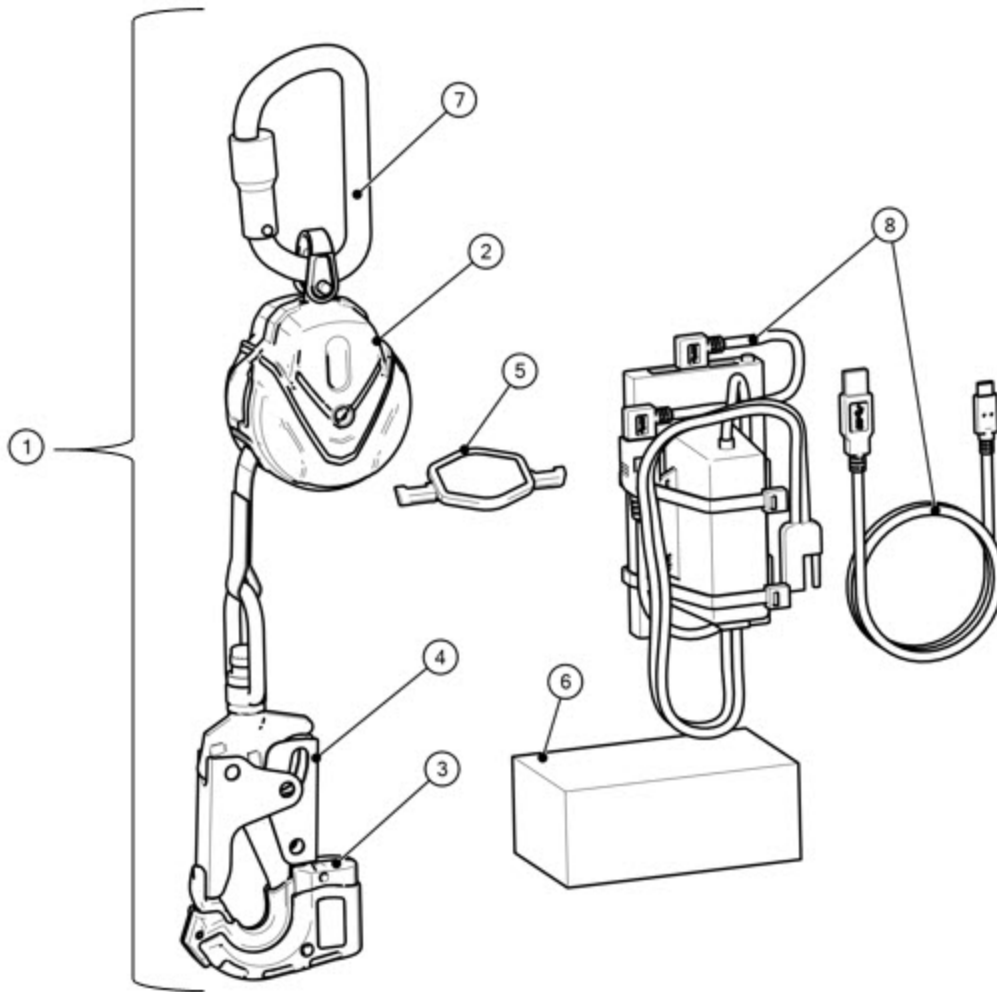
Figure 1 V-TEC io1 Components
