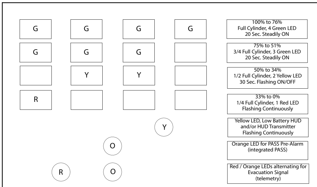
Chart 1: FireHawk M7 HUD LED Patterns for FireHawk M7XT Air Masks
