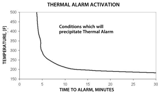
Chart 4: FireHawk M7XT Control Module Thermal Alarm Activation Curve
