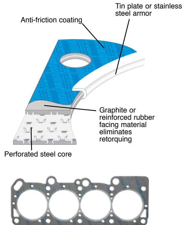
Fel-Pro PermaTorque® head gasket designs
