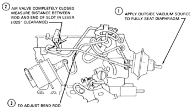
AIR VALVE ROD ADJUSTMENT
