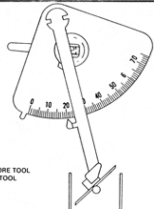
CHOKE COIL LEVER ADJUSTMENT
