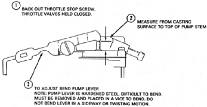
PUMP ROD ADJUSTMENT
